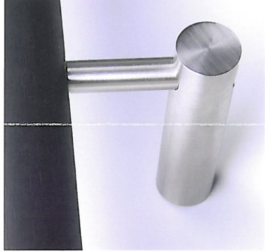
HB530 stair rail bracket machined from 316 grade stainless steel.
